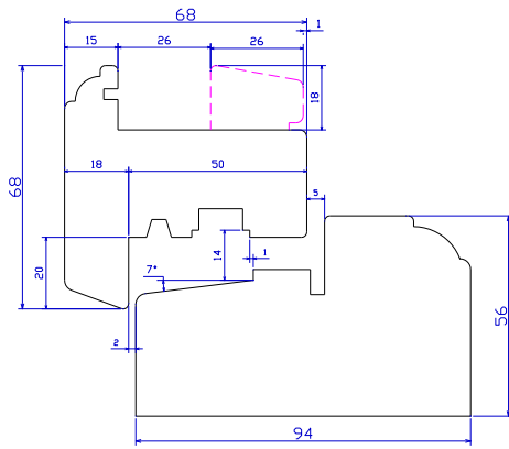
Stormproof casement window – vertical section
