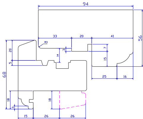
Stormproof casement window – vertical section
