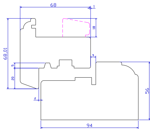
Stormproof casement window – horizontal section
